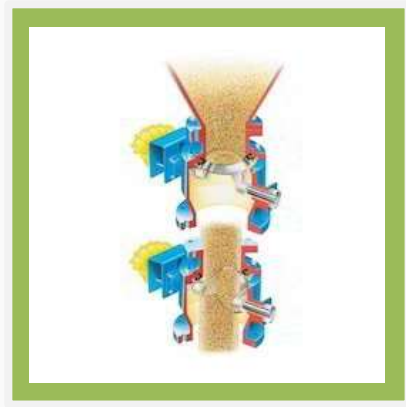
Materials Handling Dome Valve
